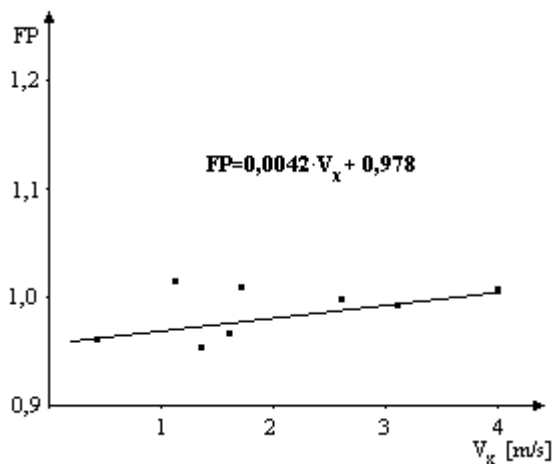
Fig. 4. The correlation between the position factor FP and pointlike velocities established for TH - arch supported mine workings
