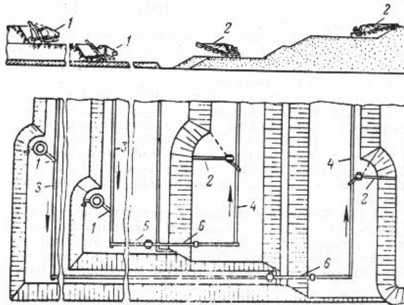
Fig. 1. Schematic representation of an open pit (1-dredge; 2-stacker; 3-transport belt conveyors; 4-stacking conveyors; 5 and 6-load and haul belt conveyor)
