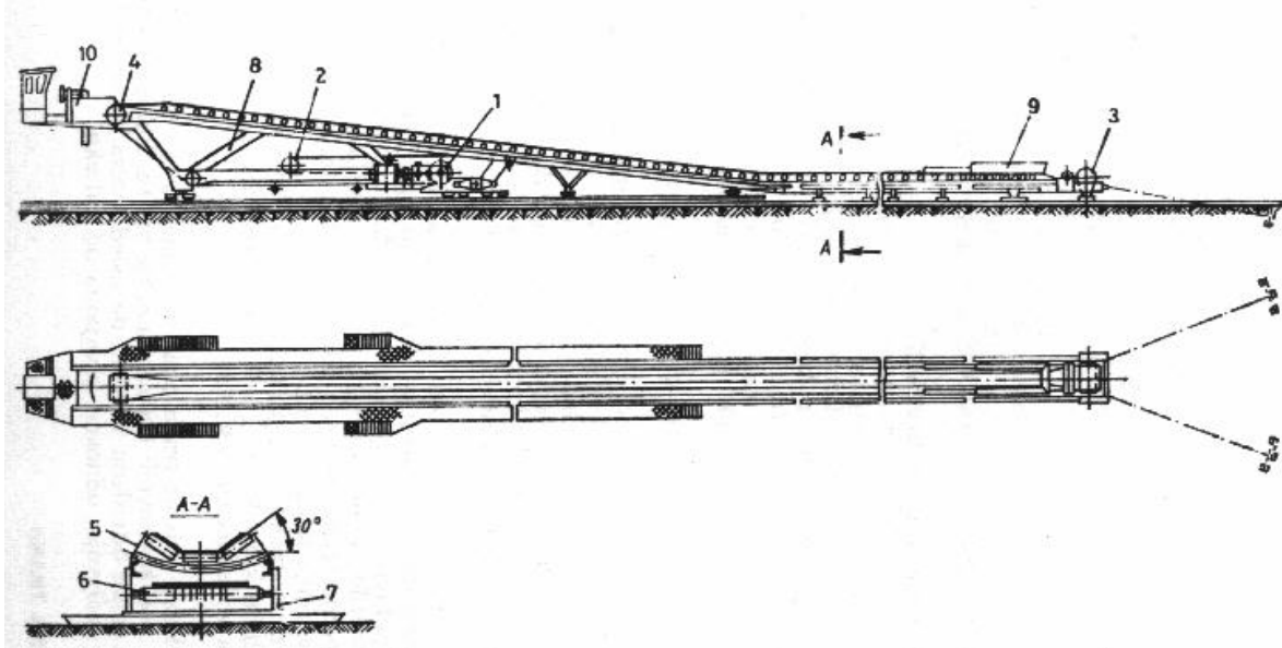
Slika 2. Schematic representation of disposition by conveyor
