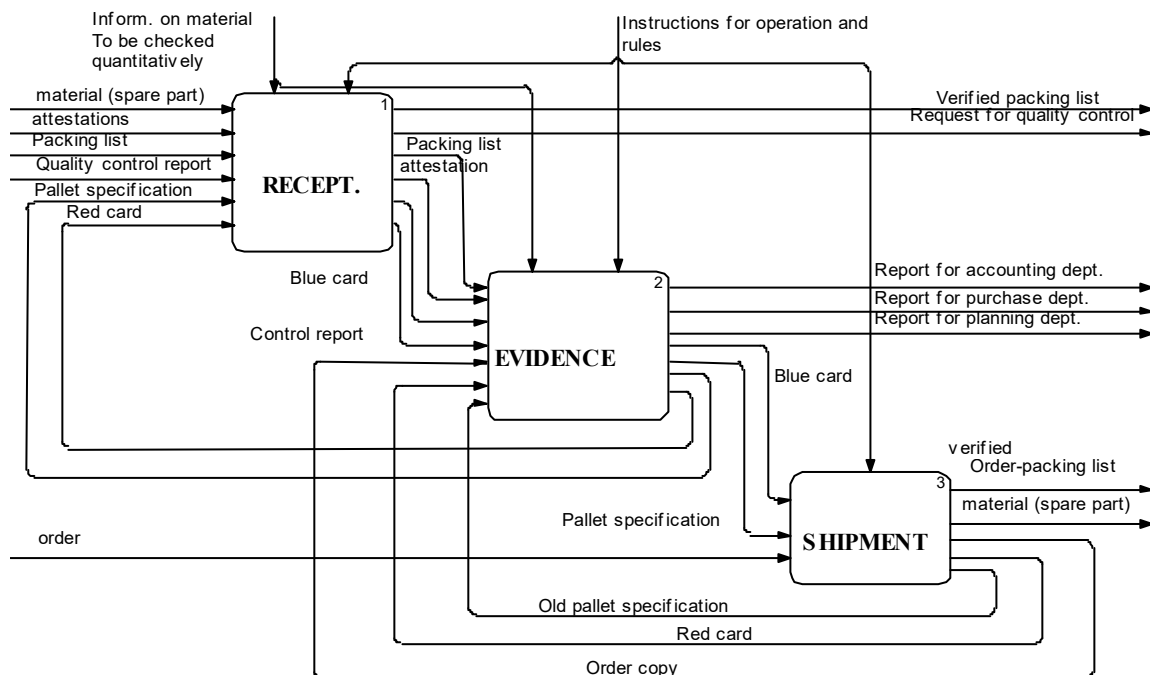
Fig. 4. Spare parts warehouse diagram
