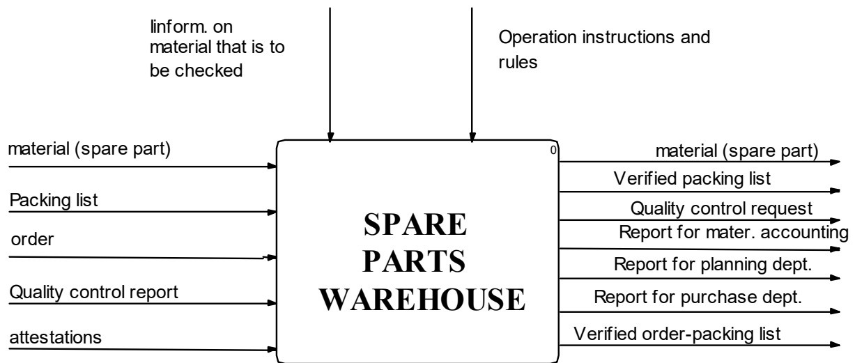
Fig. 3. Contextual diagram of a spare parts warehouse
