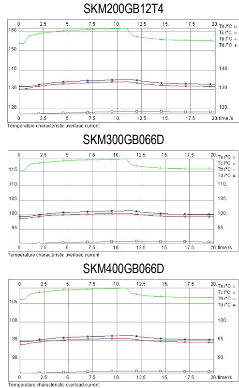
Fig. 8. Temperature losses for 3 different IGBT
