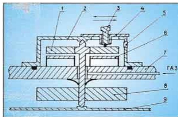
Fig. 3. A scheme for the thermochemical installation ( http://st-yak.narod.ru/index2-4-1.html ): 1 – diamond processing disk; 2 – cover; 3 – the holder with diamond; 4 – lid; 5 – observation window; 6 – heater; 7 – base; 8 – pulley; 9 – spring stress
