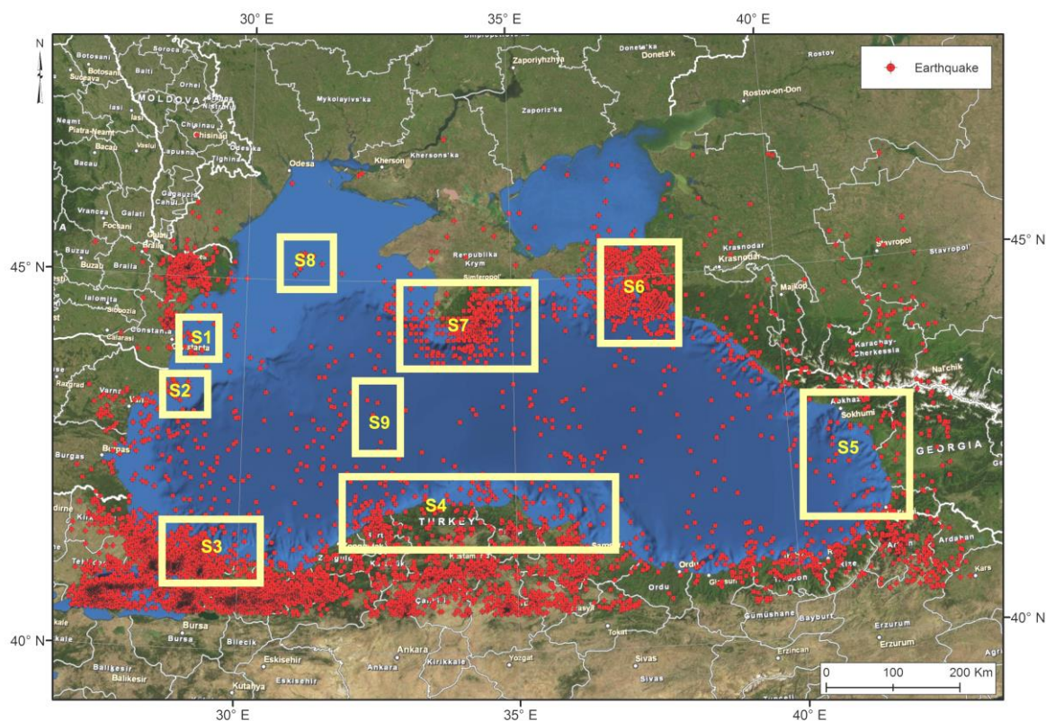
Fig. 1. Earthquakes (dots) and seismic sources (light polygons) identified as main hazard seismic zones in and around the Black Sea
