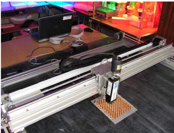
Fig. 1. Coordinate table for measuring displays
