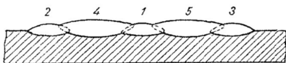
Fig. 5. Welding with narrow and wide strips
