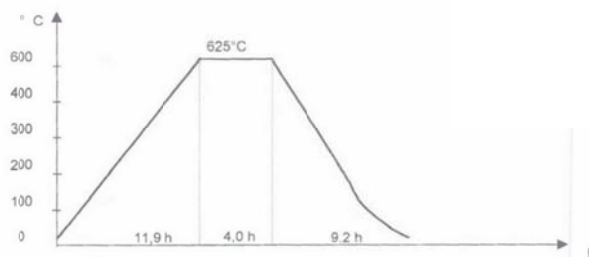
Fig. 6. Annealing characteristics
