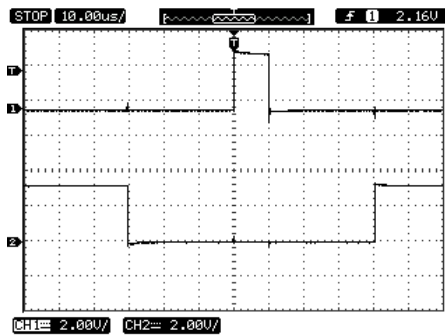
Fig. 7. Output of channels A and B for an 8-bit PWM with duty cycle of 0x02 at 100 kHz clock
