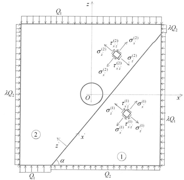
Fig. 4. Stresses in an inclined layered rock
