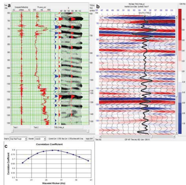
Fig. 4. Seismic line TX92-21 a/ Correlation between sonic log from P-2 Galata well and trace from the line; b/ Fragment of seismic section with synthetic trace generated from correlated P-wave curve of P-2 Galata; c/ Distribution of correlation coefficients for different frequencies of seismic impulse
