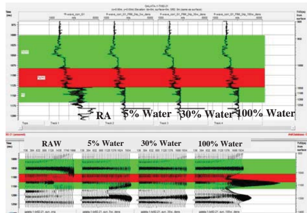
Fig. 7. AVO-modeling at water saturation 5, 30, 100%, constant density 2.22g/cm³ for target area and porosity 24% (P-1 Galata well)
