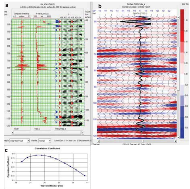
Fig. 3. Seismic line TX92-21 a/ Correlation between sonic log from P-1 Galata well and trace from the line; b/ Fragment of seismic section with synthetic trace generated from correlated P-wave curve of P-1 Galata; c/ Distribution of correlation coefficients for different frequencies of seismic impulse
