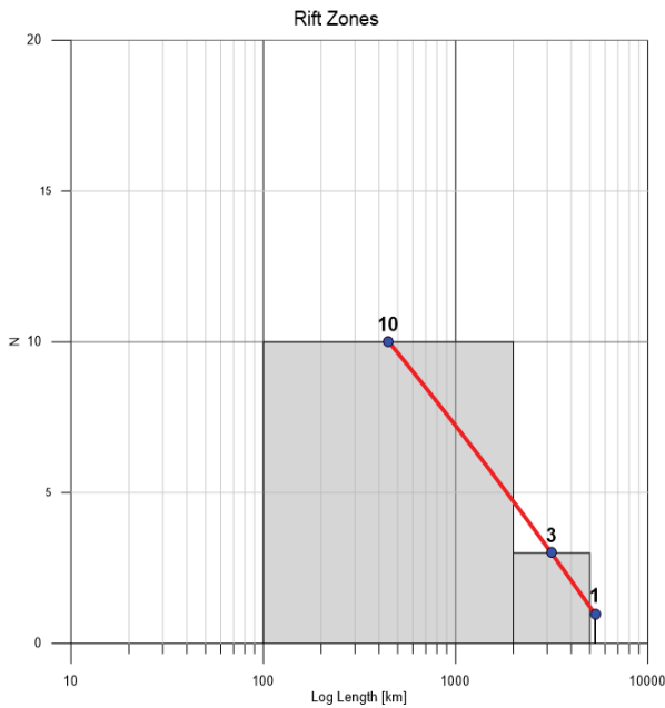
Fig. 3. Fractal distributions of the investigated rift zones.
