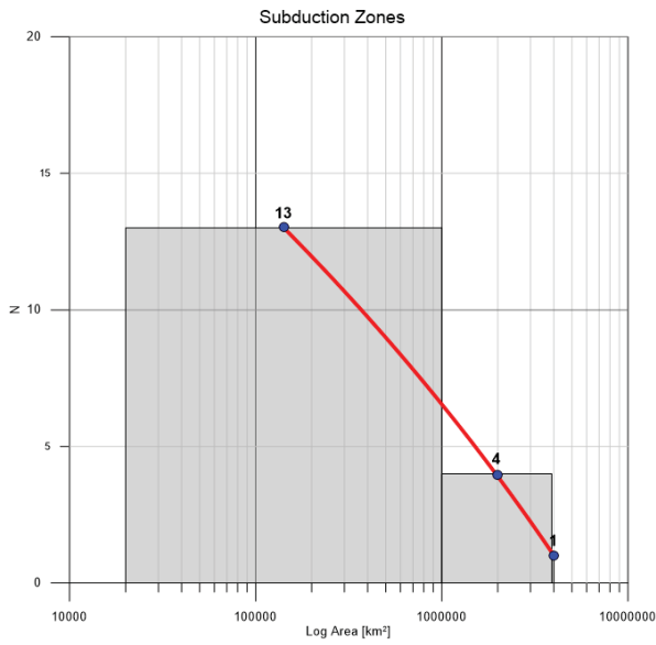
Fig. 5. Fractal distributions of the investigated subduction zones.
