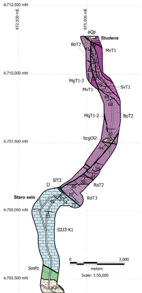
Fig. 5. Plan of the main structural elements observed at the Studena – Staro selo cross section, scale 1:50 000. SmPz – Strouma diorite Fm, SvT 1 – Svidol Fm, MgT 1-2 – Mogila Fm, PaT 1-2 – Pancharvevo Fm, BoT 2 – Bosnek Fm, RaT 2 – Radomir Fm, RdT 3 – Rusinovdel Fm, KmT 3 – Komshtitsa Fm, SIT 3 – Slaveeva Fm, IJ – Gradets, Polaten, Gintsi, Drugan Fm, IIIJ 3 -K 1 Cenral Balkan Flish Group – Neshkovo and Kostel Fm, K 2 – granodiorite porphyry, bcgOl 2 – breccia-conglomerate Fm, aQh – alluvial sediments. Bold line – fault.
