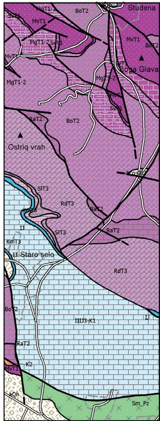
Fig. 2. Geologic map, scale 1:50 000 with amendments and supplements (Antonov et al., 2011 a, b). SmPz – Strouma diorite Fm, SvT 1 – Svidol Fm, MgT 1-2 – Mogila Fm, PaT 1-2 – Pancharevo Fm, BoT 2 – Bosnek Fm, RaT 2 – Radomir Fm, RdT 3 – Rusinovdel Fm, KmT 3 – Komshtitsa Fm, SIT 3 – Slaveeva Fm, IJ – Gradets, Polaten, Gintsi, Drugan Fm, IIIJ 3 -K 1 Cenralbalkan Flish Group – Neshkovo and Kostel Fm, K 2 – granodiorite porphyry, bcg Ol 2 – breccia-conglomerate Fm, aQh – alluvial sediments.
