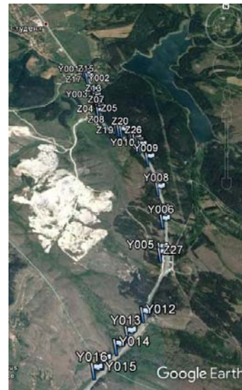
Fig. 3. Location of the Studena – Staro selo section with the waypoints.
