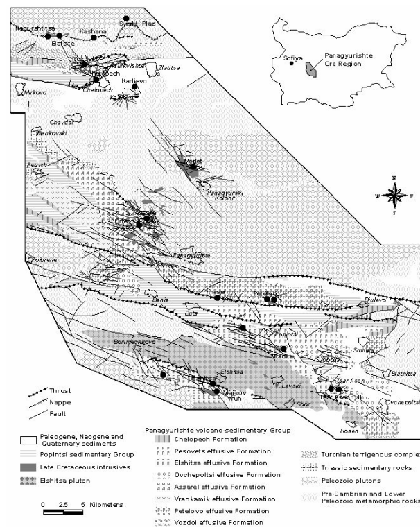
Fig. 3. Geological map of the Panagyurishte ore region (Popov, 2005)
