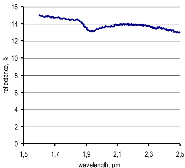
Fig. 4. Plot showing ASTER spectra of granite (Baldrige et al., 2009)
