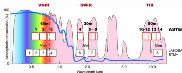
Fig. 2. ASTER bands ( http://asterweb.jpl.nasa.gov/images/spectrum.jpg , June 2016)
