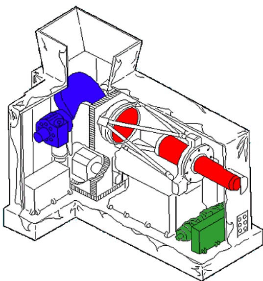
Fig. 1. ASTER Instrument Subsystem SWIR ( http://asterweb.jpl.nasa.gov/swir.asp , June 2016)
