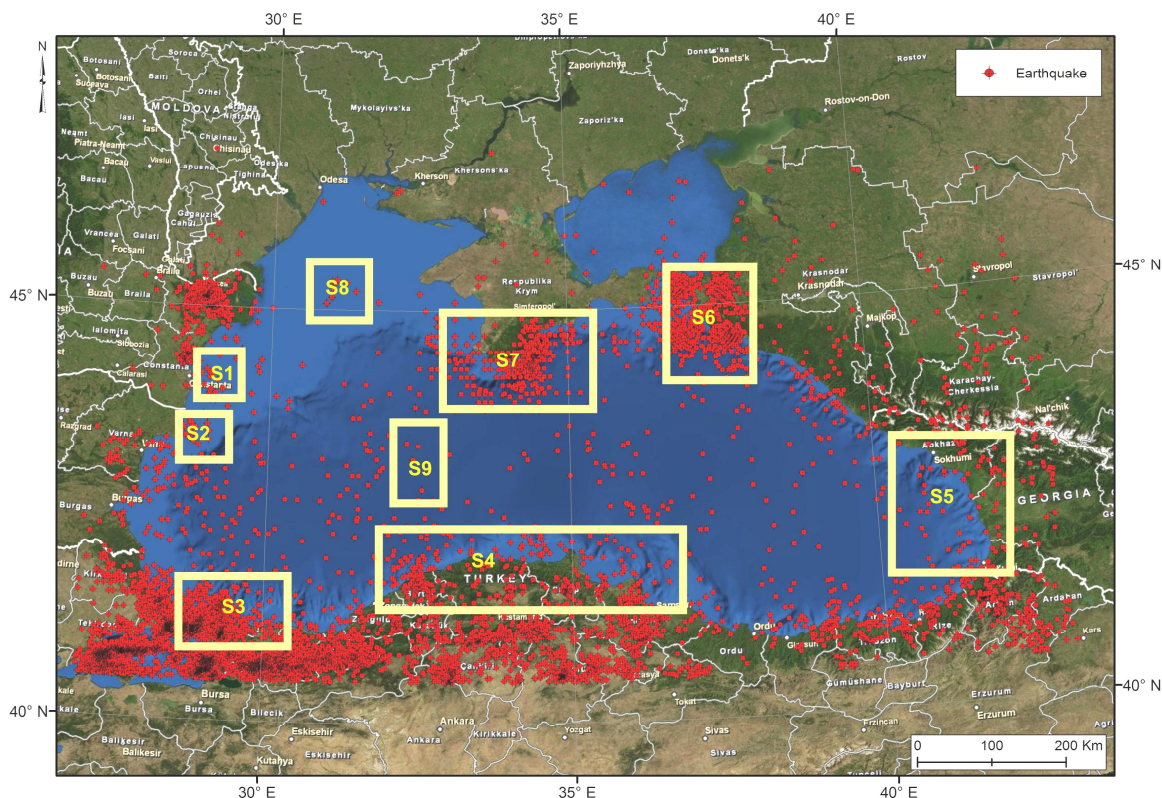
Fig. 1. Earthquakes (dots) and seismic sources (light polygons) identified as main hazard seismic zones in and around the Black Sea
