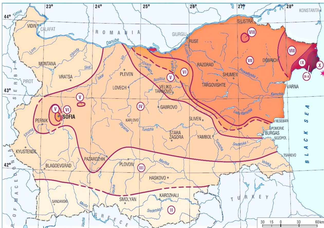
Fig. 4. Macroseismic map of the earthquake from 31 March, 1901
