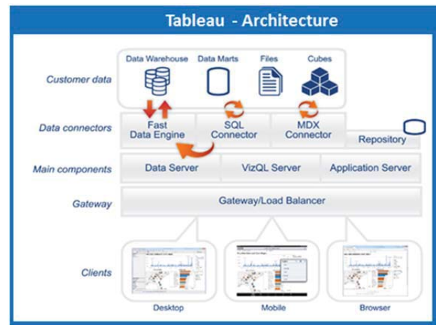
Fig 3. Tableau Architecture
