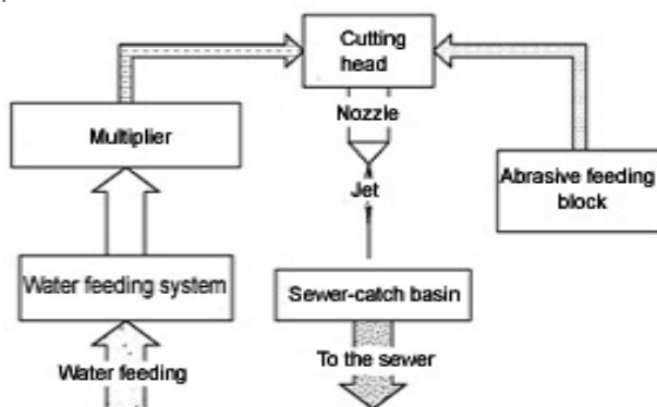
Fig. 3. Functional relation of the water jet modules.
