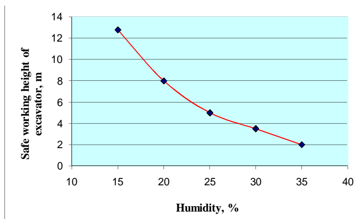
Fig. 4. Dependence of the safe working height of the excavator on the humidity of tailings
