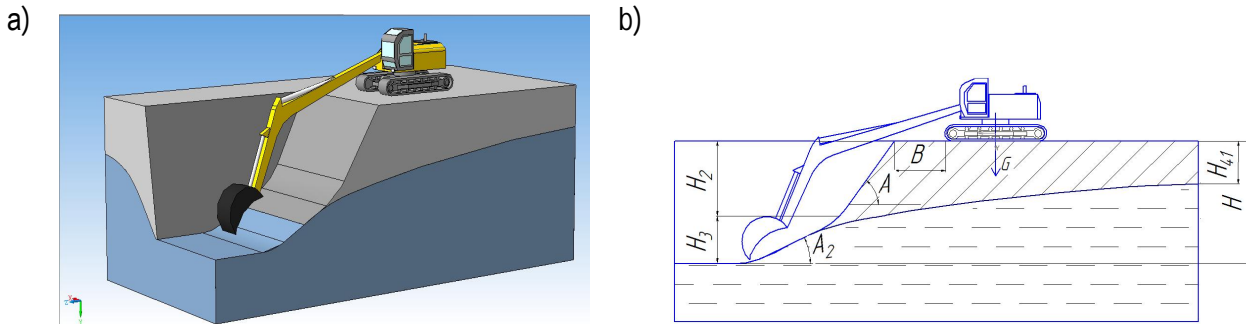
Fig. 1. Computer-aided simulation of processes taking place in the gravel face during the operation of the back-acting excavator: a) 3D-model; b) 2D-model.
