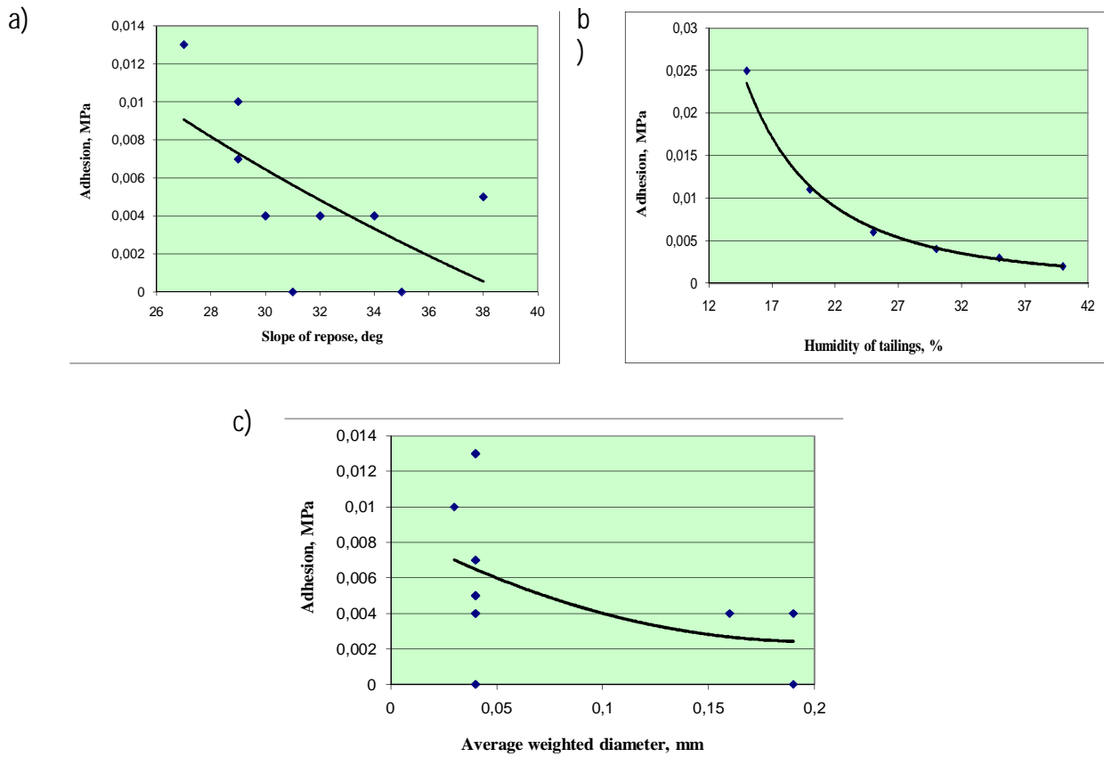
Fig. 3. Graphs of dependence of physical and mechanical properties of iron-bearing stale tailings: a) adhesion on slope of repose; b) adhesion on humidity of stale tailings; c) adhesion on average-weighted diameter of tailings.
