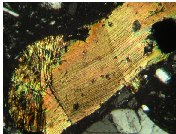
Fig. 3. Microscope image of thinsection from the grey rhyolites (image size 1.5 mm) deformed biotite crystal
