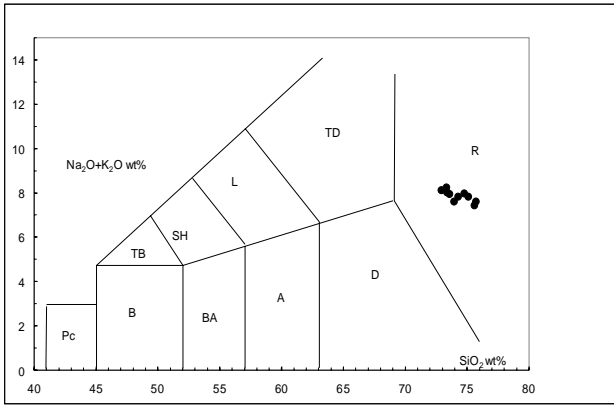
Fig. 5. TAS diagram after Le Maitre (1989) for representative samples from the studied region (B – basalt; BA – basaltic andesite; A – andesite; D – dacite; SH – shoshonite; L – latite; T D – trachydacite; R – rhyolites)
