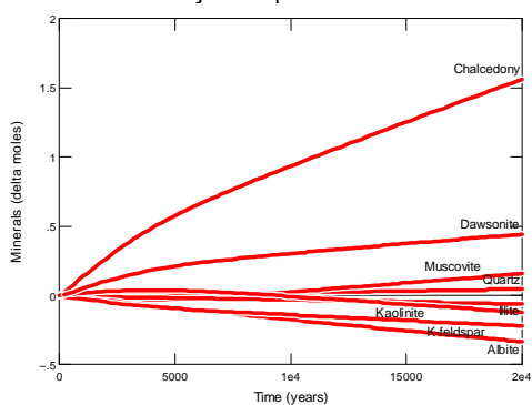
Fig. 8. Changes of minerals quantities in 20ka after the injection termination – D5 sample – the injection point
