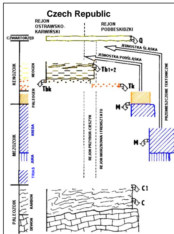
Fig. 2. Hydrostratigraphical profile of the Czech part of the USCIB (after Labus, Grmela, 2003): Q – Quaternary complex; T_b , T_{b1+2} – waters of Lower Badenian sandy horizons within clayey cover of the Carboniferous complex (Skawina Formation); T_{bk} – waters of sandy-gravel sediments of Lower Badenian (Dębowiec Formation); T_k – waters of sandy and sandstone aquifers of autochthonous Carpatian; M – fissure waters of the Subsilesian Nappes; C_1 – fissure and pore waters of Carboniferous; C – waters of fissure-fault system of upper Carboniferous and its basement. Arrows indicate the possibility of groundwater downward migration into the deeper aquifers
