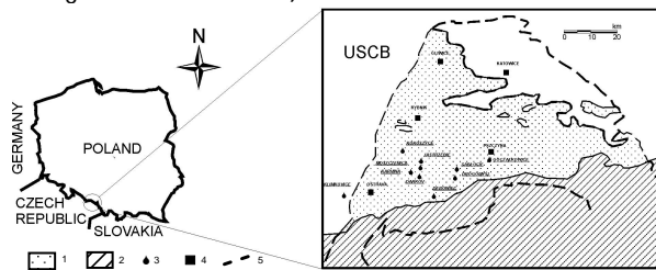
Fig. 1. The Upper Silesian Coal Basin – USCBB (Labus, Grmela, 2003): 1 – Tertiary overburden; 2 – Carpathians; 3 – medicinal waters exploitation; 4 – towns; 5 – borders of the USCBB
