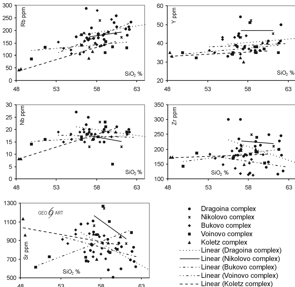
Fig. 2. Diagrams showing distribution of Rb, Nb, Y, Zr, Sr in rocks from Sarnitsa Group
