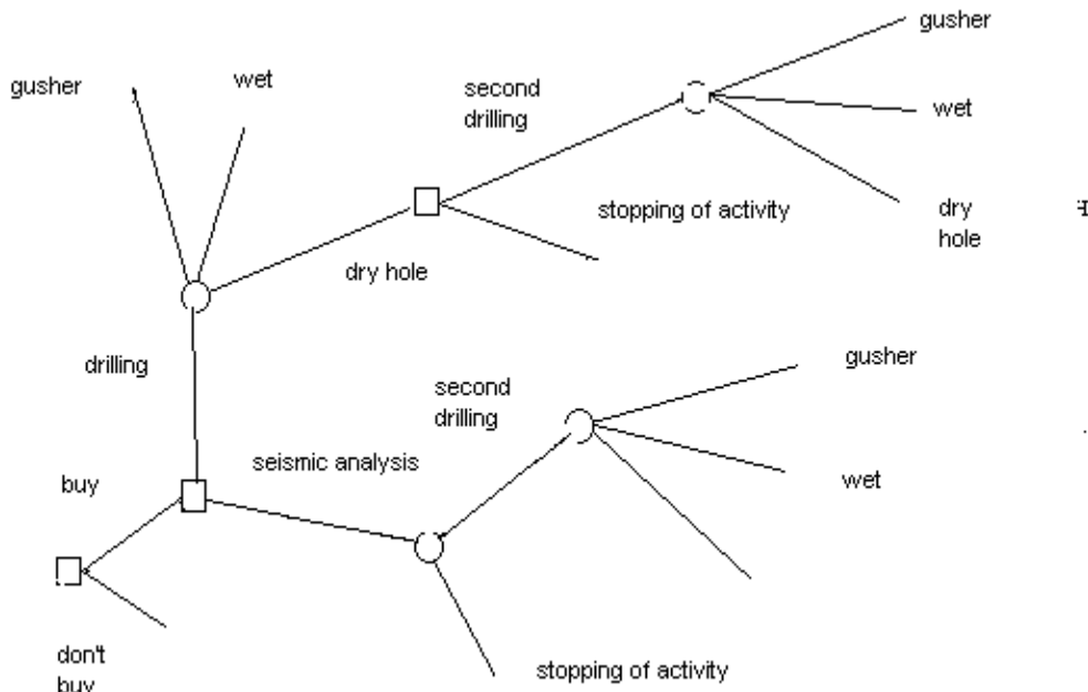
fig.1 Decision tree
